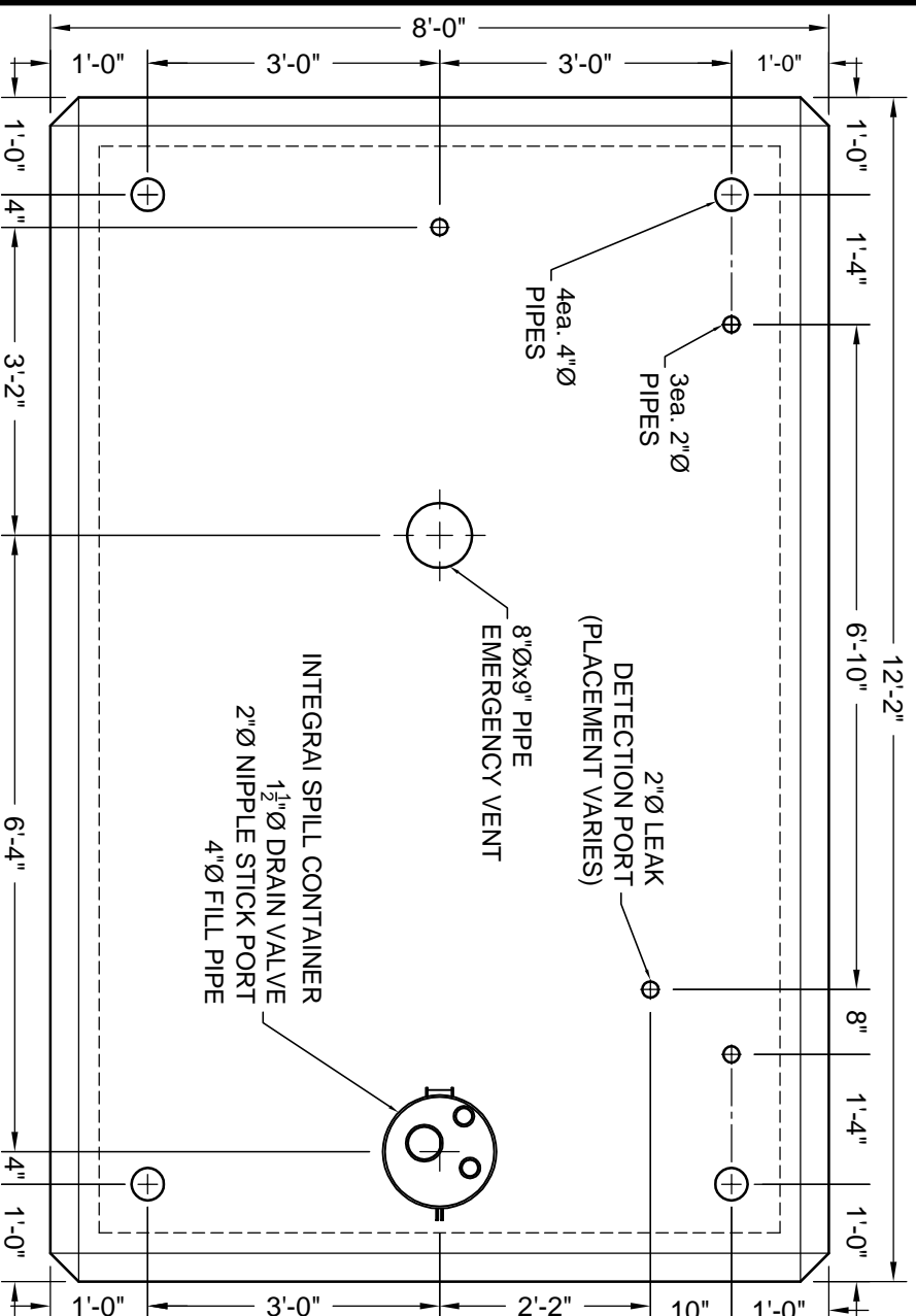
TYPICAL PLAN VIEW
